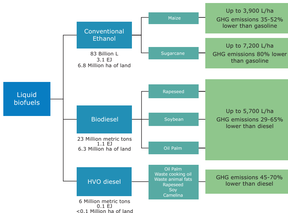
Figure 2.1. Current feedstocks and biofuels. Approximate numbers.
