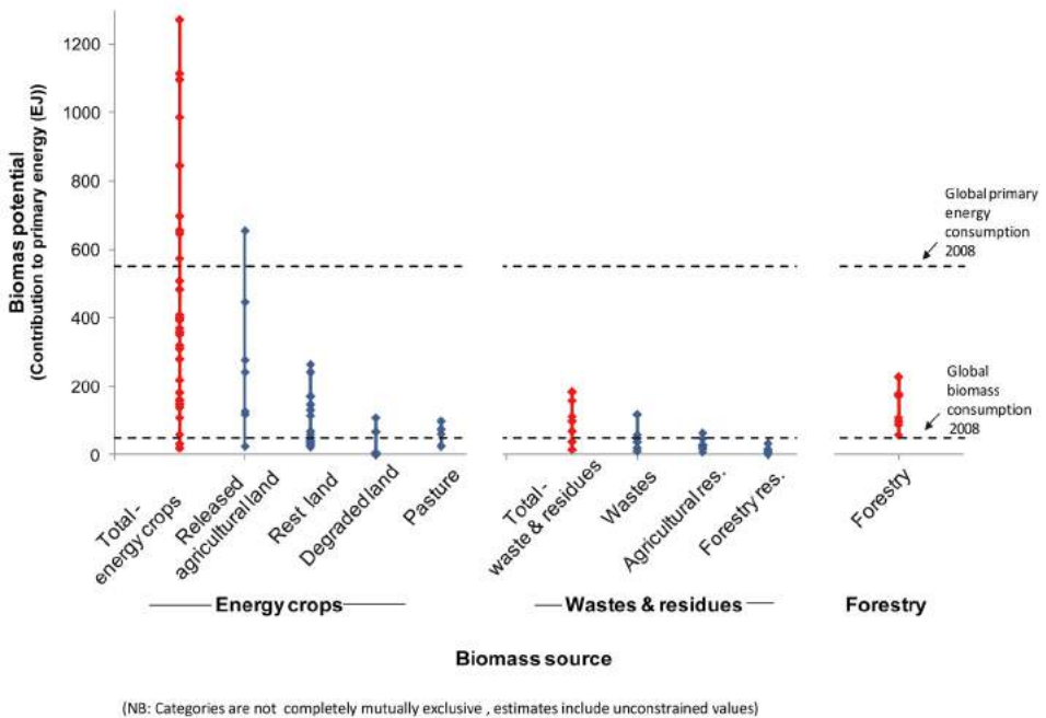
Figure 9.12. Bioenergy supply potentials based on meta-analysis of 28 global studies (Slade et al. 2014).
